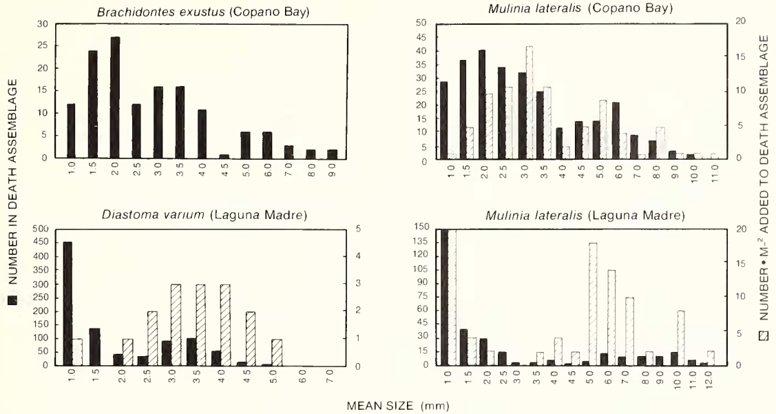
TEXT-FIG. 6. Comparison of the average size-frequency distribution in the death assemblage and the calculated size-frequency distribution of living individuals that died during the study period for taxa with bimodal distributions. Number in the death assemblage is the total number actually collected during the study.
